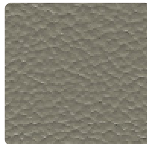
Shale
