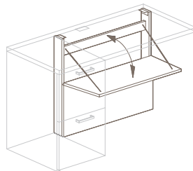
Hinged panel detail
