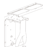
CPU holder CPUH-1
