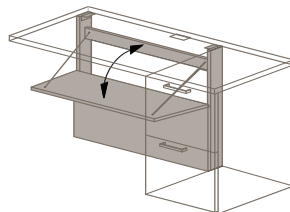
Optional hinged access panel for full height back panels (FLFZ)
