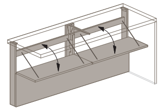
48.0625"w-94"w fold down door detail
