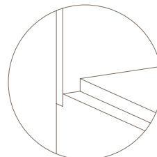
Wall panel recesses behind surface
