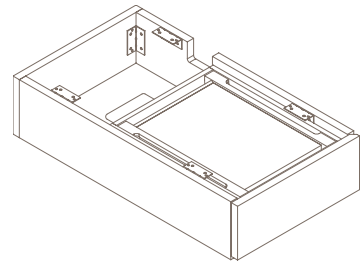
C5P tech drawer
