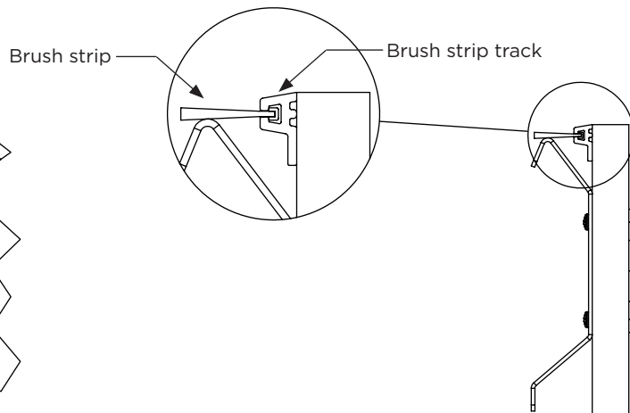
Elevation C
