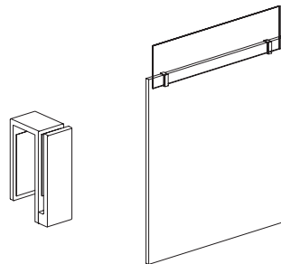
PVPBKT-1 bracket
